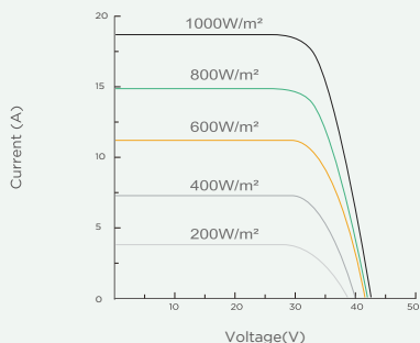
Current-Voltage Curve(SP605M-60H)
