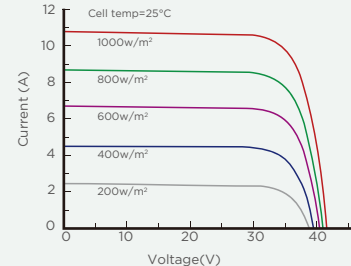
Current-Voltage Curve(SP450M-60H)
