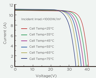
Current-Voltage Curve(SP450M-60H)
