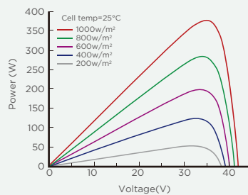
Current-Voltage Curve(SP450M-60H)
